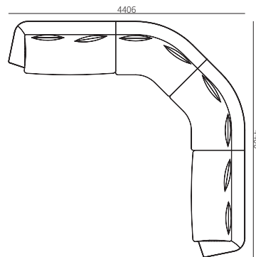
31F006ZH-08 4406*4400*755mm 173.5*173.2*29.7"
