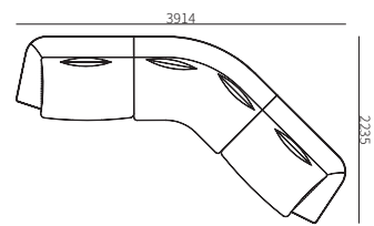
31F006ZH-06 3914*2235*755mm 154.1*88.0*29.7"
