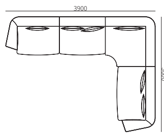
31F006ZH-05 3900*3000*755mm 153.5*118.1*29.7"
